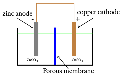
Figure 3: A zinc copper Galvanic cell with aqueous solutions of \text{ZnSO}_4 and \text{CuSO}_4 separated by a porous membrane. When active, sulfate anions \text{SO}_4^{2-} flow across the membrane from the copper side to the zinc side.
